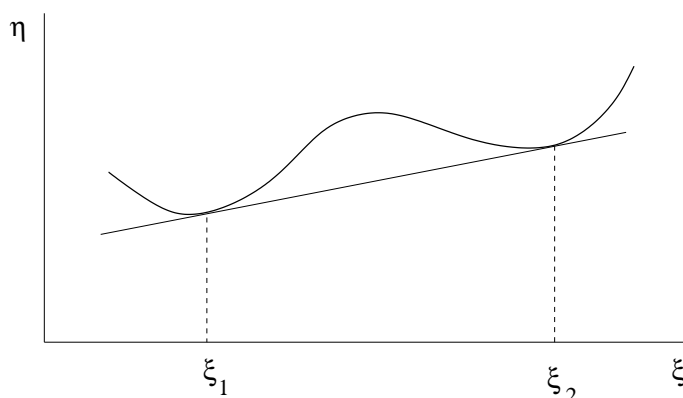
Figure 3.8: Geometric meaning of the Corollary
