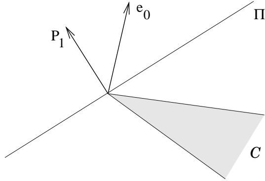
Figure 3.18: Separation of \mathcal{C} and L = re_0
