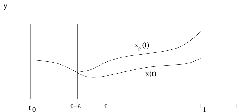
Figure 3.16: Variation of the trajectory
