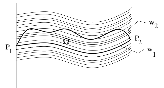
Figure 3.14: Proof of Lemma 3.3.2
