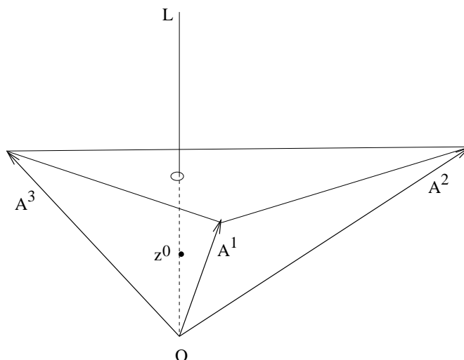
Figure 3.19: Simplex in consideration
