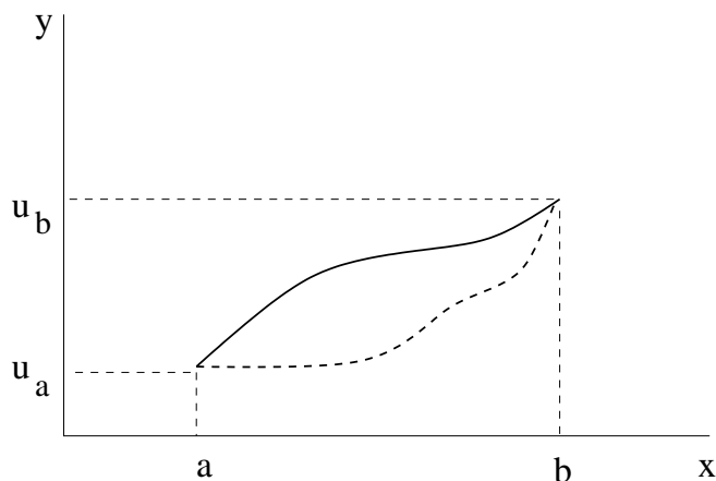
Figure 3.1: Admissible variations
