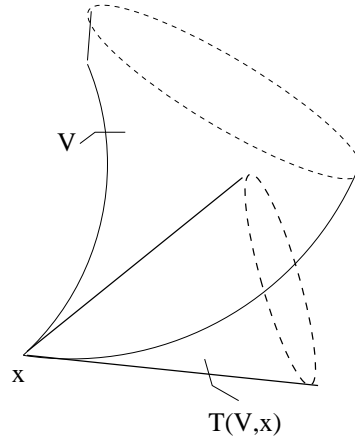
Figure 2.2: Tangent cone
