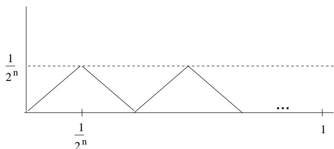
Figure 3.5: Nonsmooth solutions
