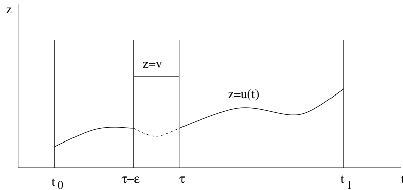
Figure 3.15: Needle variation
