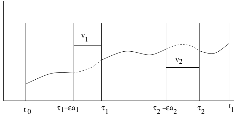
Figure 3.17: Needle variations
